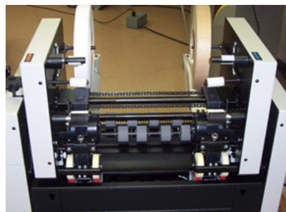
5002-KT2 Tabber Head 1 and 2 adjusted for wide tab placement
